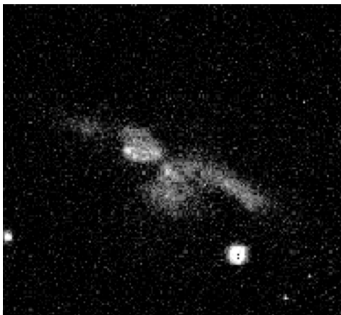
Ultraviolet – I (ASTRO-1 UIT)
