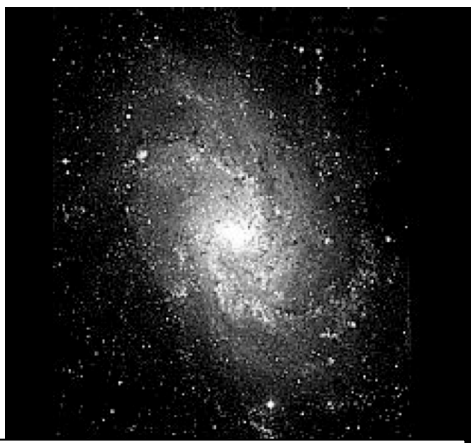
Visible - 5 (IAC/RGO/Malin)
