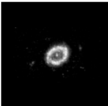
Ultraviolet – VII (ASTRO-2)
