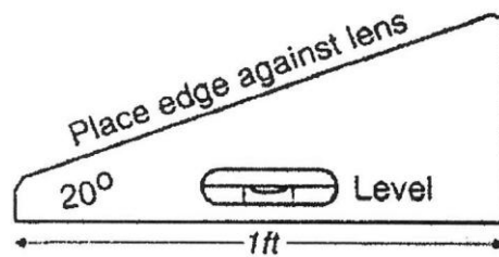
EXHIBIT 2: A tool for aiming lights as in Exhibit 1. Place the upper edge of the tool against the lens and adjust the fixture so the bubble shows level.
